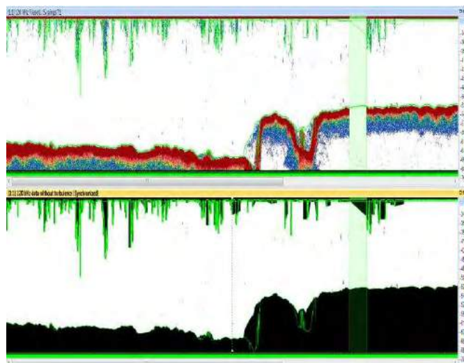
Fig. 3 Snapshot of an echogram from the August survey, first ebb tide, transect N1 against the tide (raw data, top and data corrected without turbulence, bottom) where the reverse bottom detection processing method has been performed. The analysed portion of the echogram corresponds to the white part of the echogram between the two black sections in the bottom echogram shown
