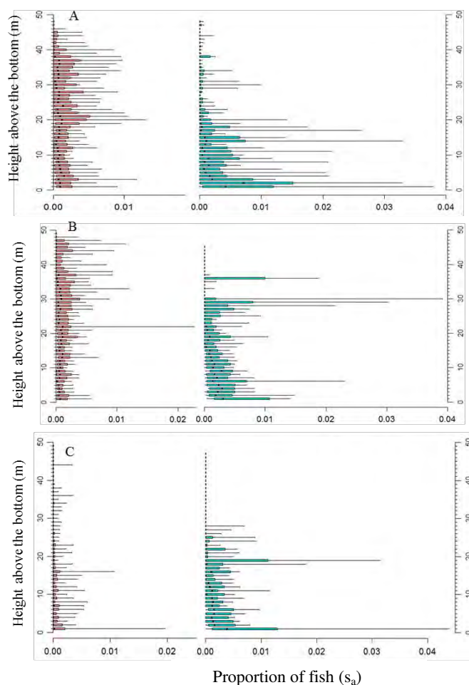
Fig. 7 Boxplot of proportion of the relative fish density ( s_a ) by 1m depth layer for November 2016 (A), January (B) and March (C) 2017 after the turbine deployment and by site (CLA in red, left and reference in blue, right). The proportion of s_a (x axis) is very small reflecting the high variability and the fact that outliers (big fish or fish aggregations which can represent a high percentage of the total fish density) have not been plotted to be able to see trends in vertical distributions
