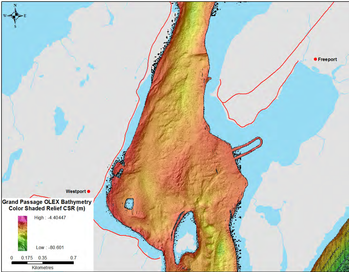
Figure 17: Olex multibeam coverage, color shaded relief (CSR) image for Grand Passage.
