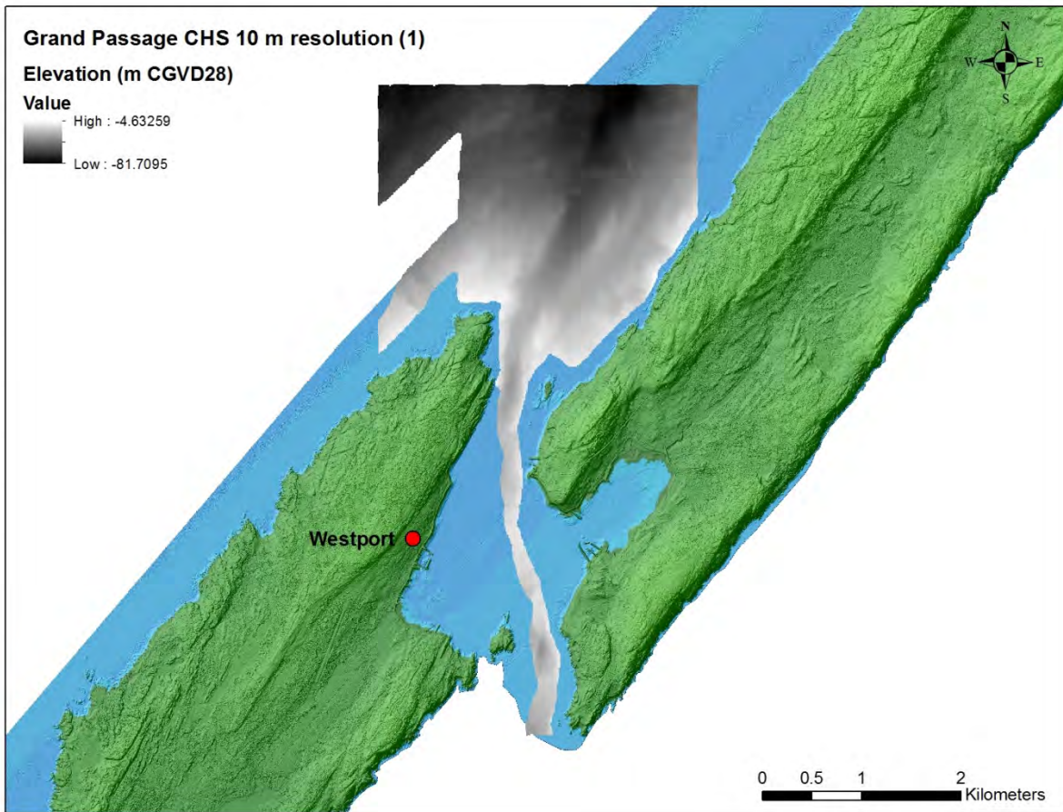
Figure 2: Grand Passage CHS 10 m multibeam bathymetry data, courtesy of Glen King (CHS).
