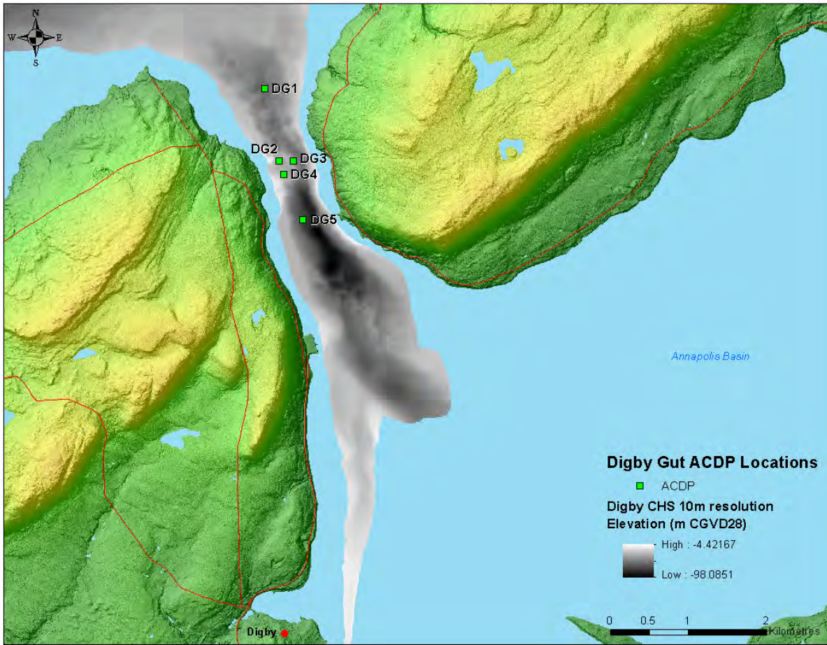
Figure 21: Location of ACDP deployment in Digby Gut.
