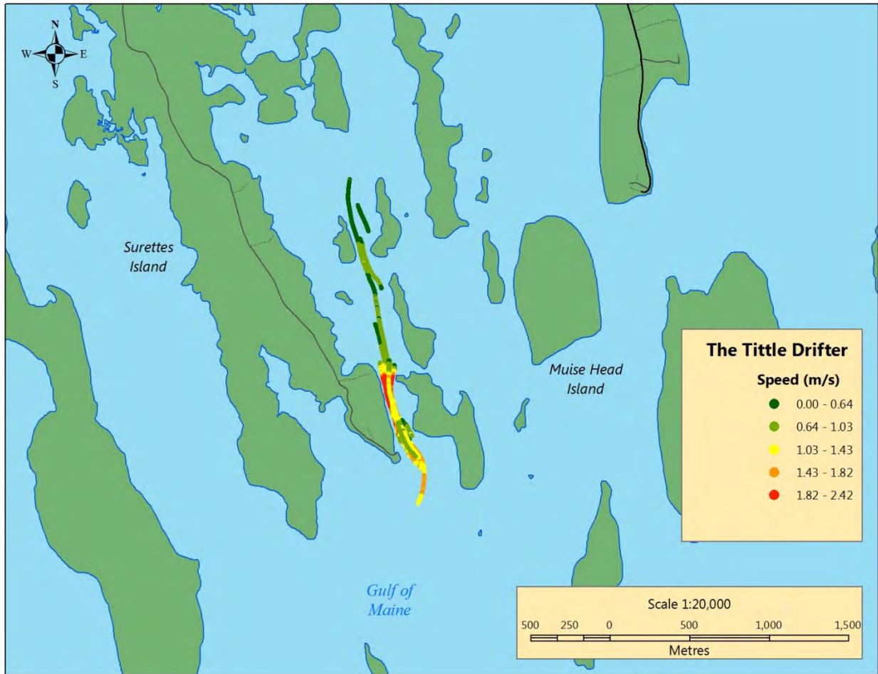
Figure 24 Drifter speed plot near the Tittle channel.
