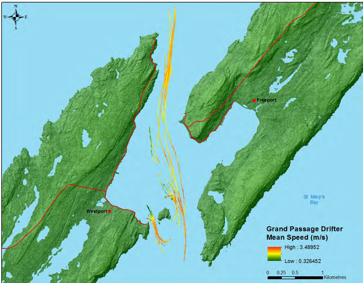
Figure 24: Drifter Mean Speed (m/s) in Grand Passage
