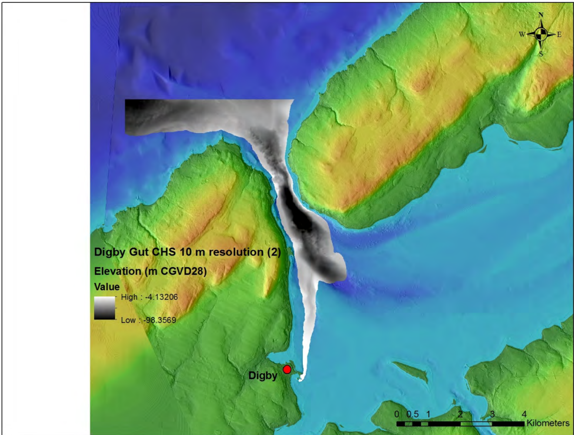
Figure 9: Digby Gut CHS 10 m multibeam bathymetry data, courtesy of Greg Towse.
