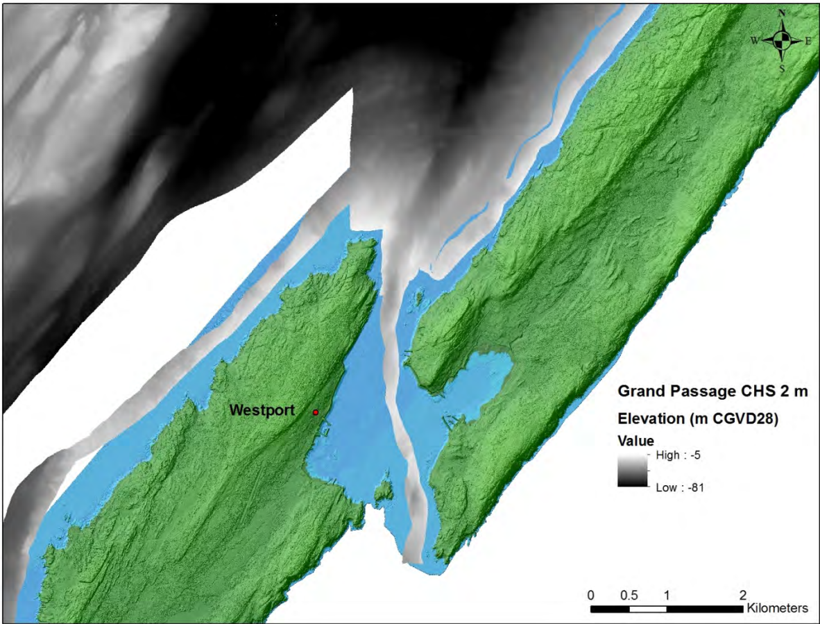
Figure 12: Grand Passage CHS 2 m grid.
