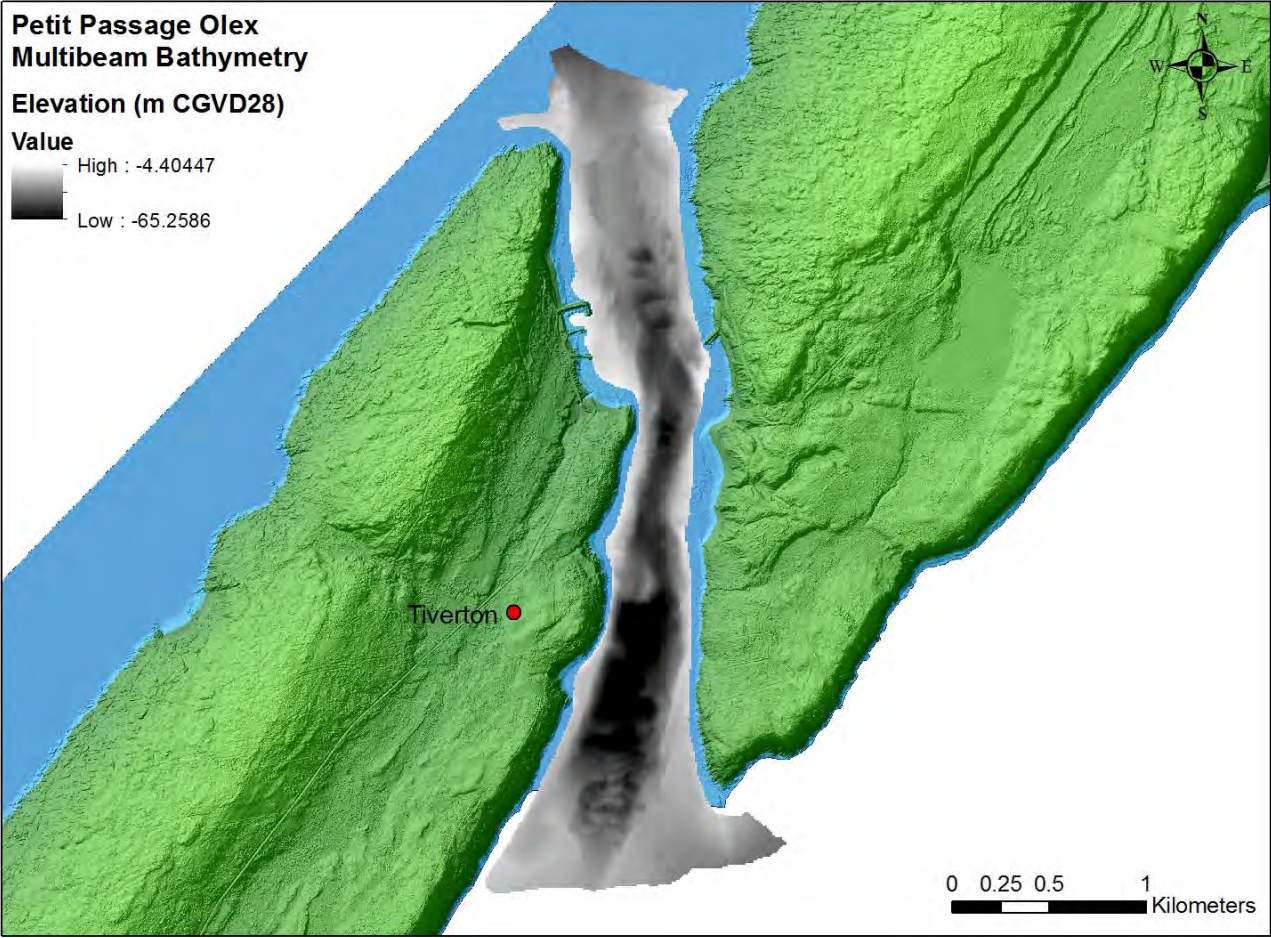
Figure 15: Olex multibeam coverage for Petite Passage.
