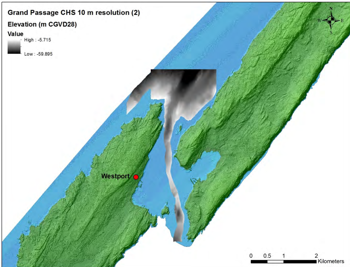
Figure 3: Grand Passage CHS 10 m multibeam bathymetry data, courtesy of Greg Towse.
