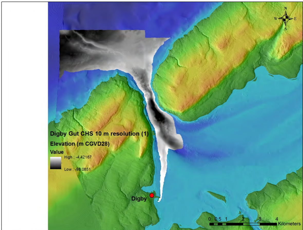
Figure 8: Digby Gut CHS 10 m multibeam bathymetry data, courtesy of Glen King (CHS).
