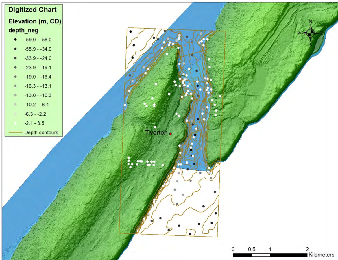
Figure 20: Digitized Chart for Petite Passage.
