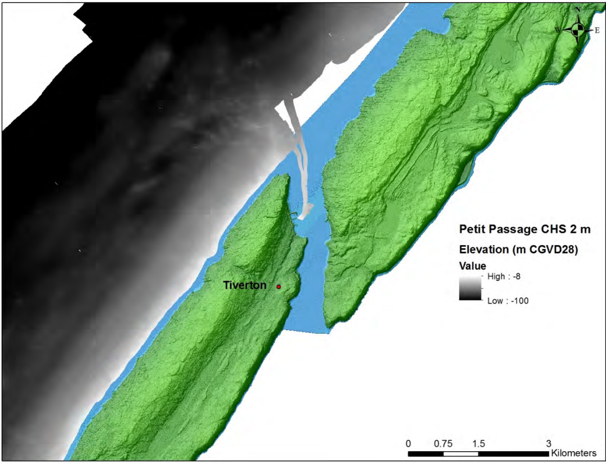
Figure 13: Petite Passage CHS 2 m grid.
