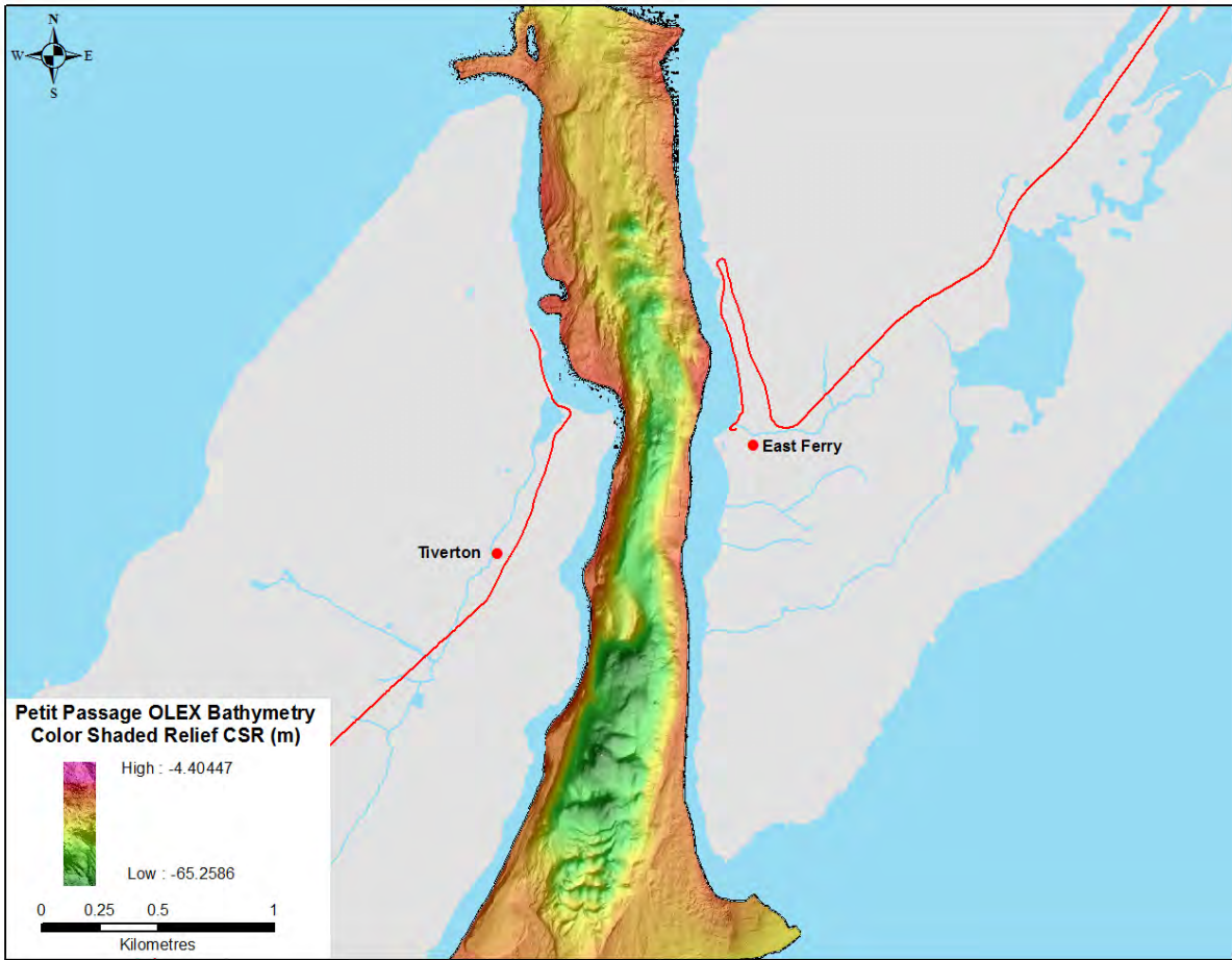
Figure 16: Olex multibeam coverage, color shaded relief (CSR) image for Petite Passage.
