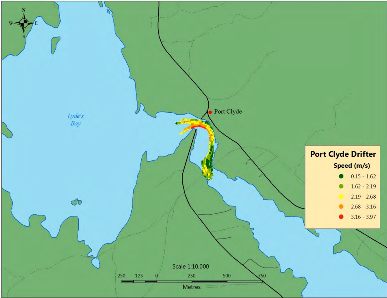
Figure 28 Drifter speed plot near port Clyde.
