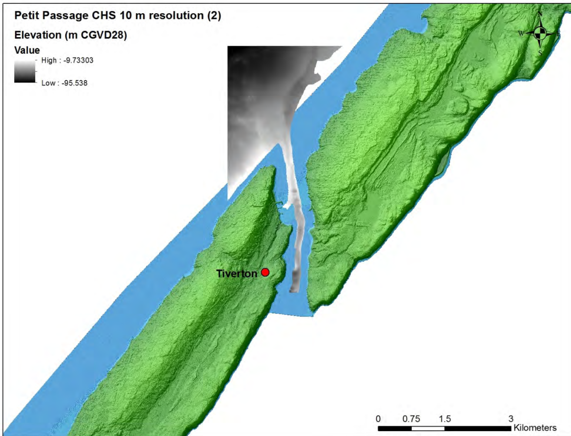
Figure 6: Petit Passage CHS 10 m multibeam bathymetry data, courtesy of Greg Towse.
