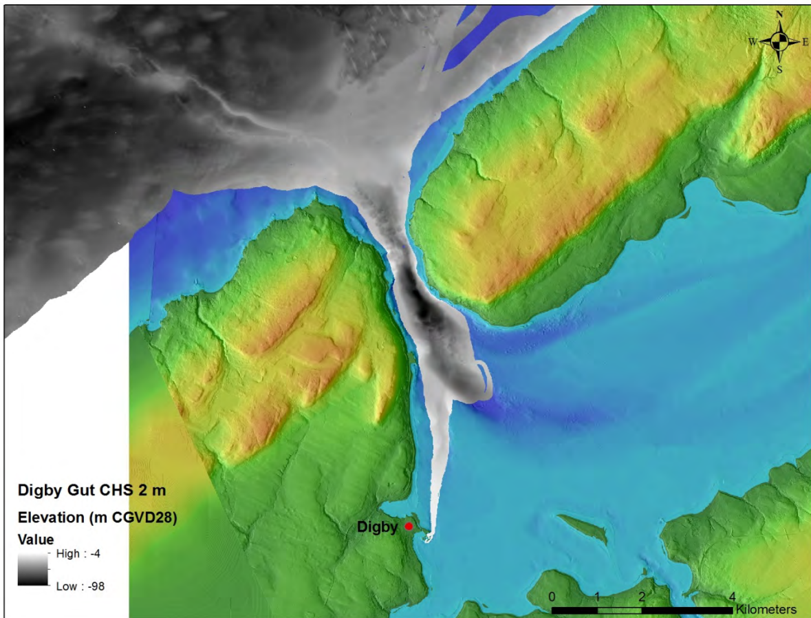
Figure 14: Digby Gut CHS 2 m grid.
