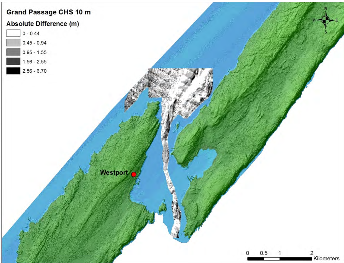
Figure 4: The absolute value of the difference between the two different CHS 10 m datasets at Grand Passage; maximum difference is 6.7 m.
