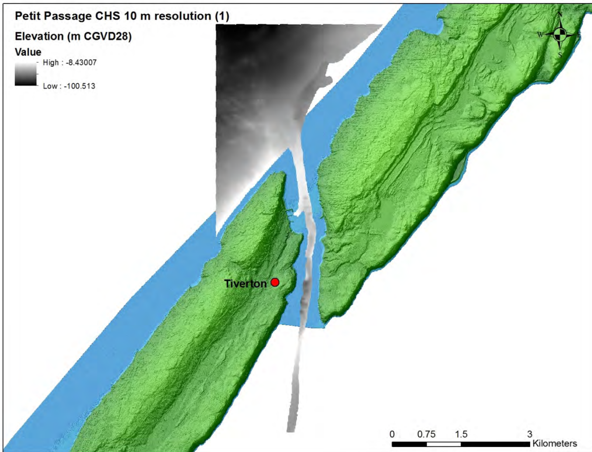
Figure 5: Petit Passage CHS 10 m multibeam bathymetry data, courtesy of Glen King (CHS).
