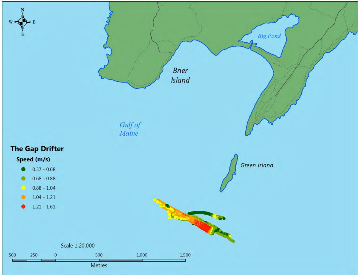
Figure 22 Drifter speed plot of “The Gap” near Green Island.
