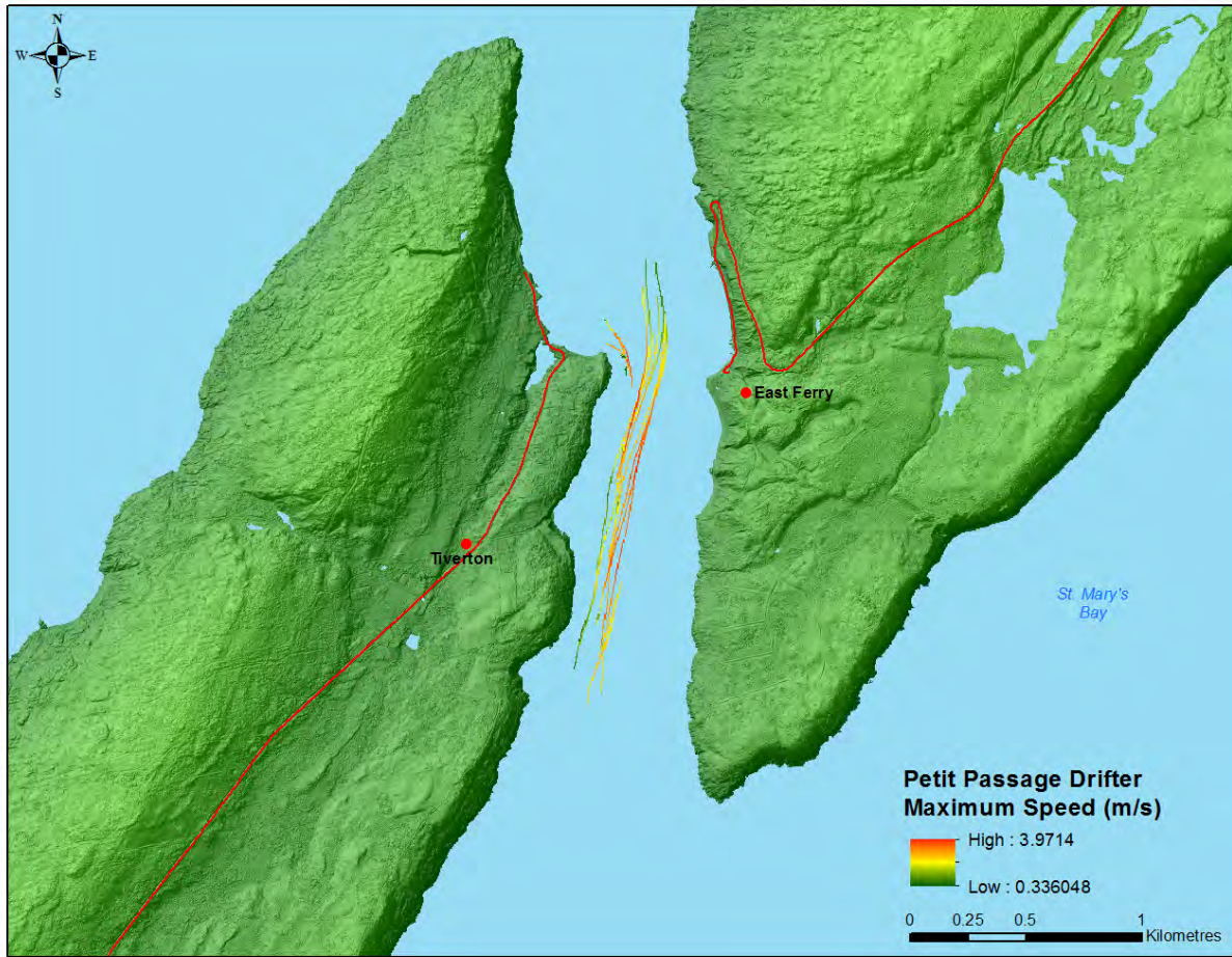
Figure 28: Drifter Maximum Speed (m/s) in Petit Passage
