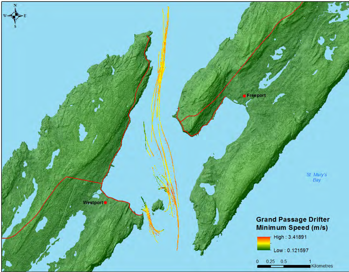
Figure 26: Drifter Minimum Speed (m/s) in Grand Passage.
