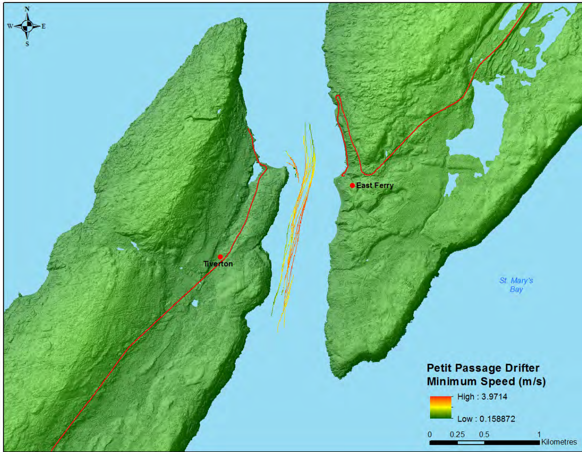
Figure 29: Drifter Minimum Speed (m/s) in Petit Passage
