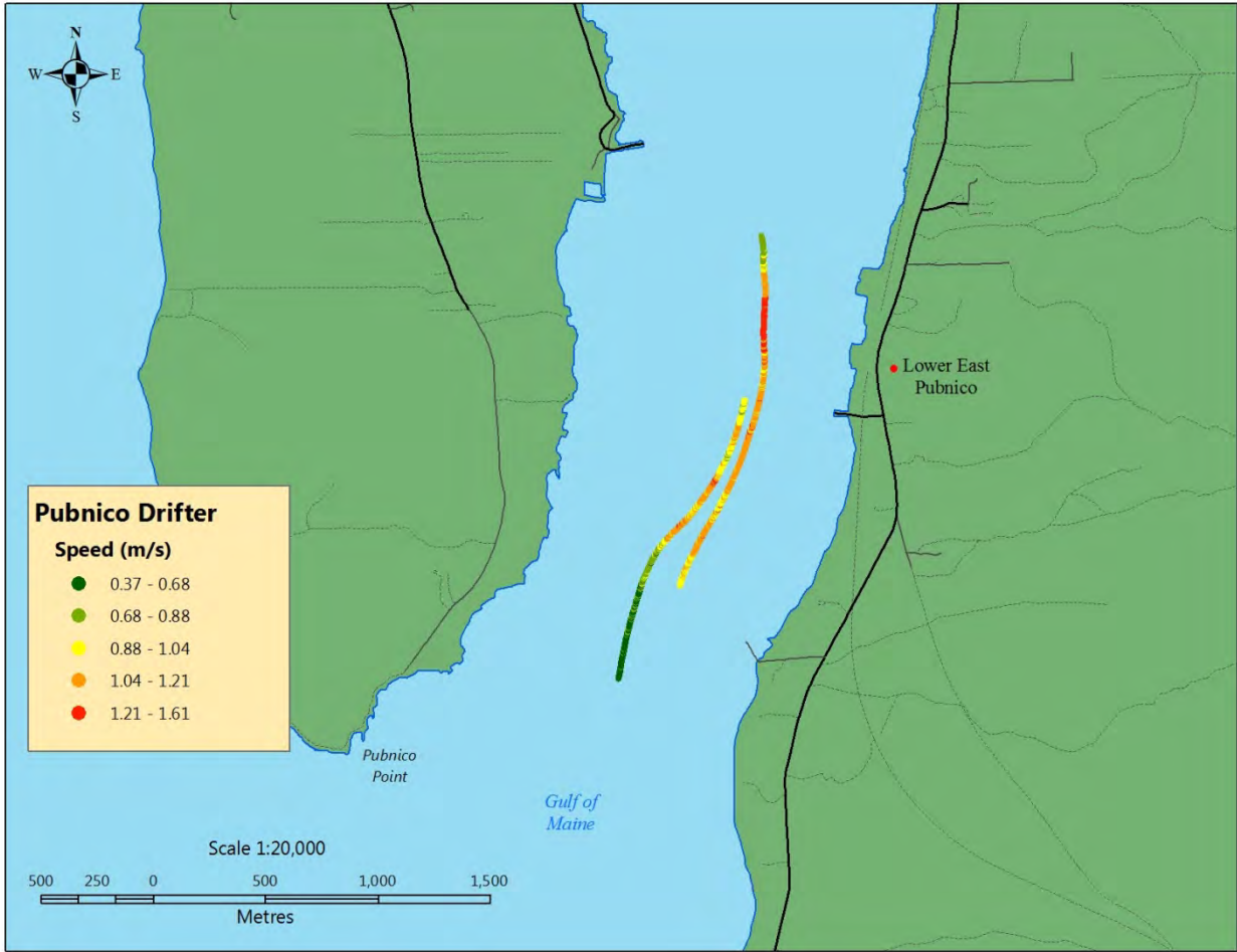
Figure 27 Drifter speed plot near Lower East Pubnico.
