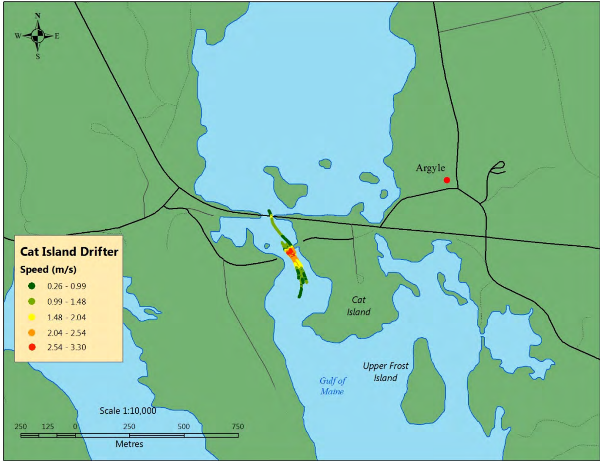
Figure 26 Drifter speed plot of the Cat Island channel.
