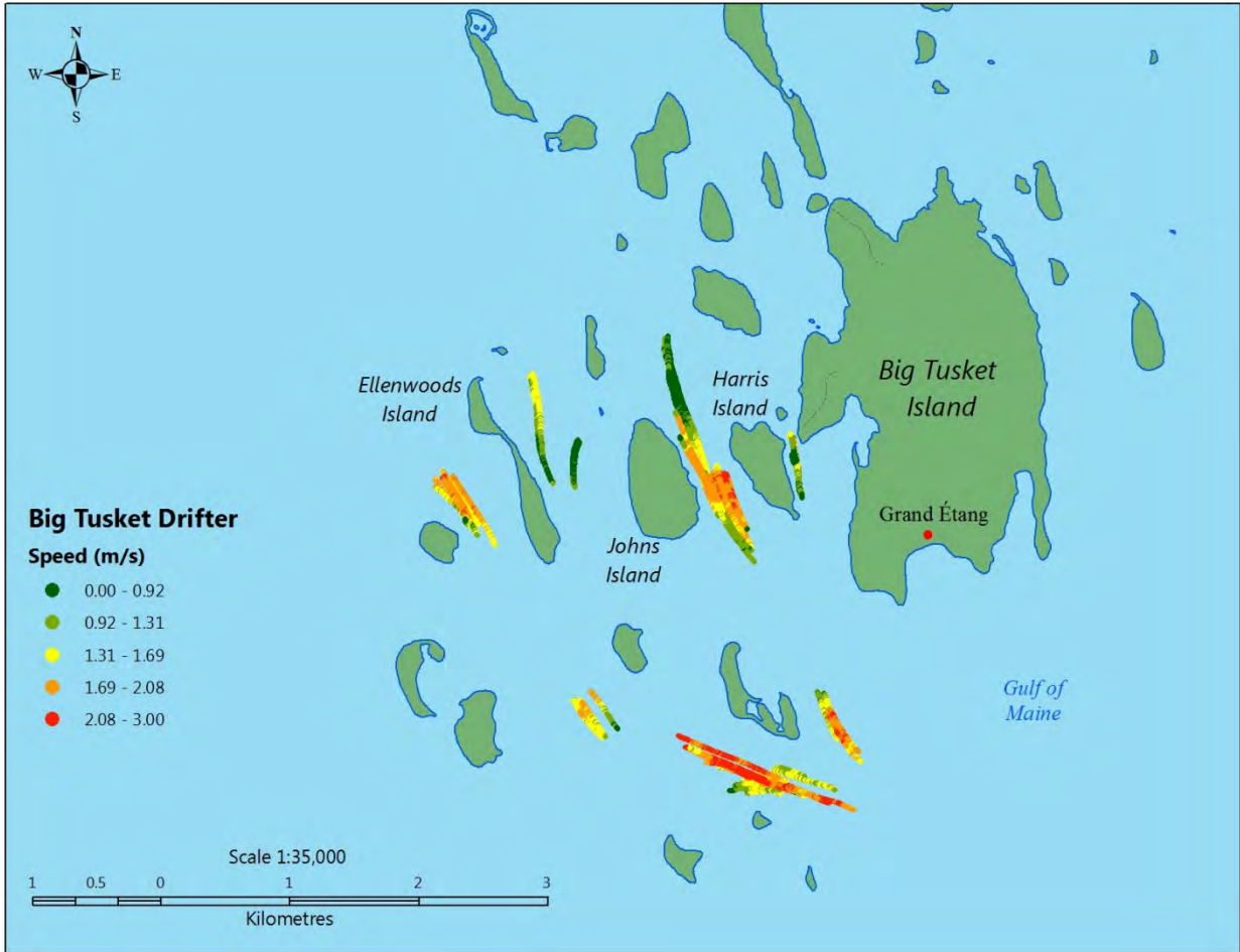
Figure 23 Drifter speed plot near Big Tusket Island.
