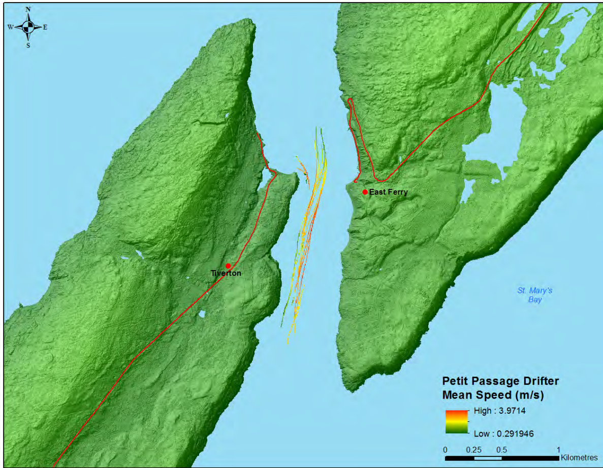
Figure 27: Drifter Mean Speed (m/s) in Petit Passage.
