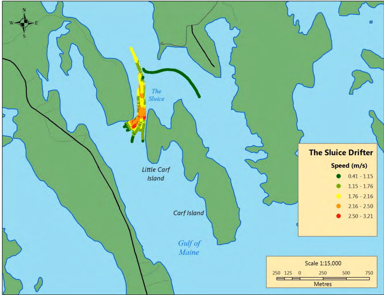
Figure 25 Drifter speed plot of “The Sluice”.
