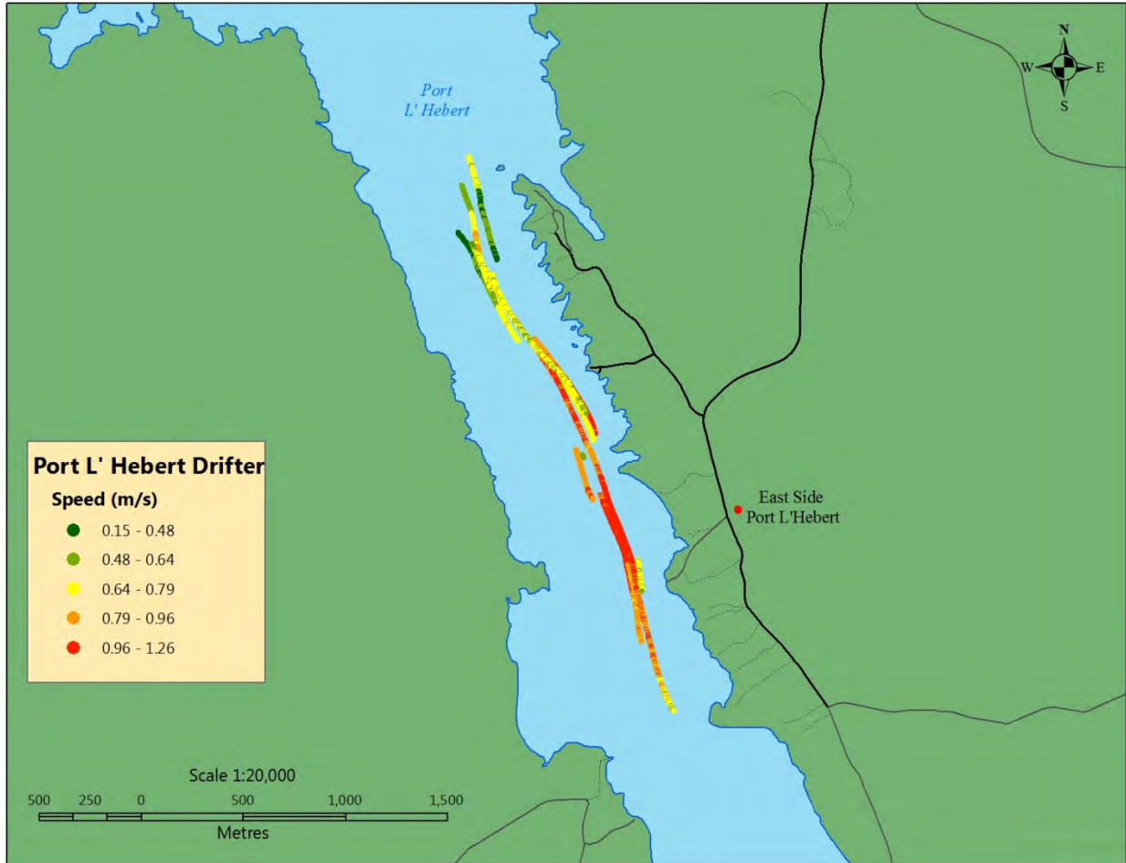
Figure 29 Drifter speed plot near Port Hebert.
