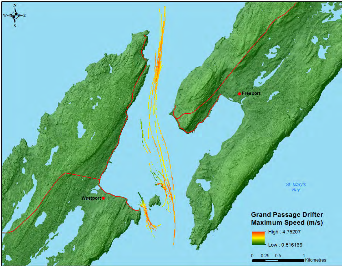
Figure 25: Drifter Maximum Speed (m/s) in Grand Passage.
