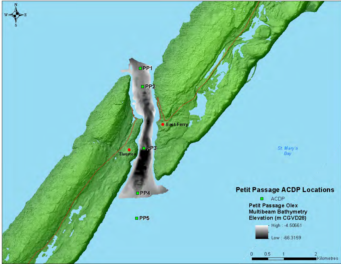
Figure 20: Location of ACDP deployment in Petit Passage.
