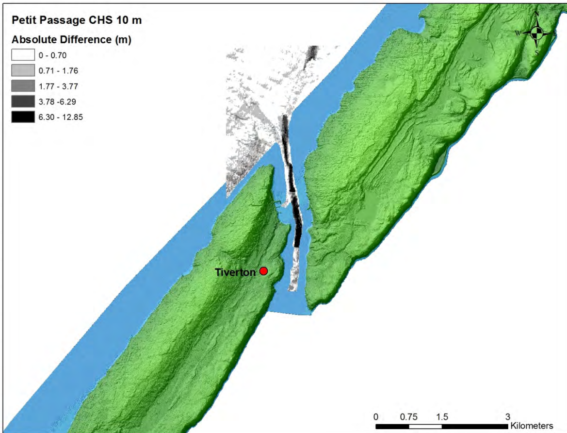
Figure 7: The absolute value of the difference between the two different CHS 10 m datasets at Petit Passage. Differences up to 12.85 m exist within the deep channel.
