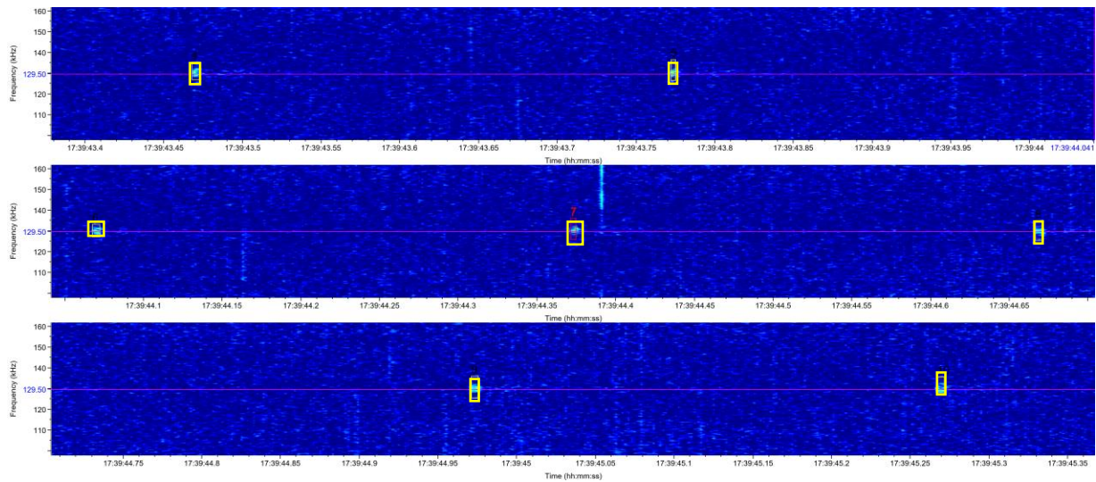
Figure 8: Spectrogram (FFT = 2048, 50% overlap, 512 kHz sample rate) from the bottom-mounted hydrophone during passive drifts showing received pseudo clicks (yellow boxes), and a 130 kHz reference line (purple) used for aiding in the click detection process. Lack of impulsive sounds facilitated easier detection of pseudo clicks.
