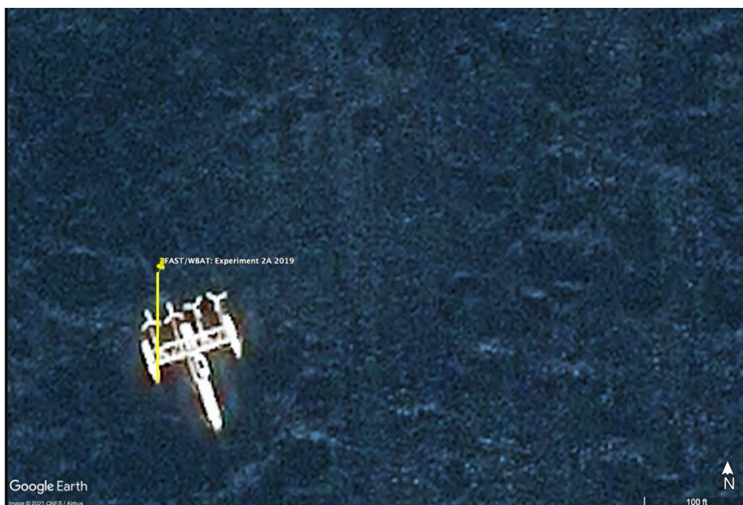
Figure 3.2.2: Deployment location of the WBAT echosounder mounted on the FAST platform, shown for Study 2A relative to the PLAT-I on a flooding tide. Length of yellow line represents the horizontal length from the optical camera deployed at the leading edge of the starboard pontoon to the position of the FAST platform: ~30 m.
