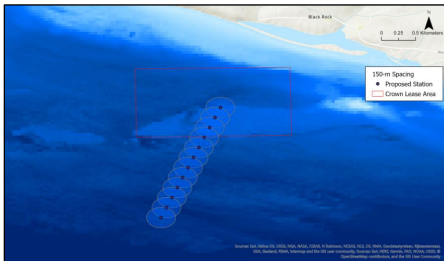
Figure 7: Acoustic receiver array deployment configuration in Minas Passage.
